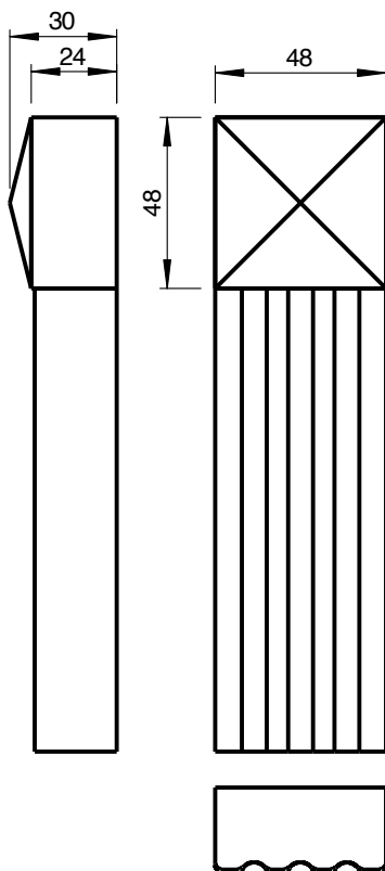
Pilaster
